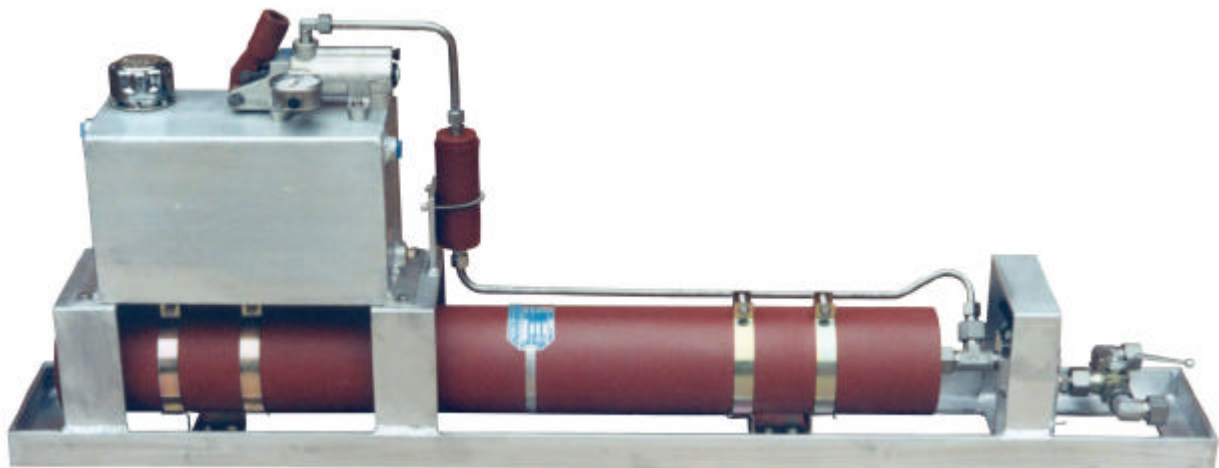
HPS starting system with all components mounted on a frame. The system is made out of stainless steel
